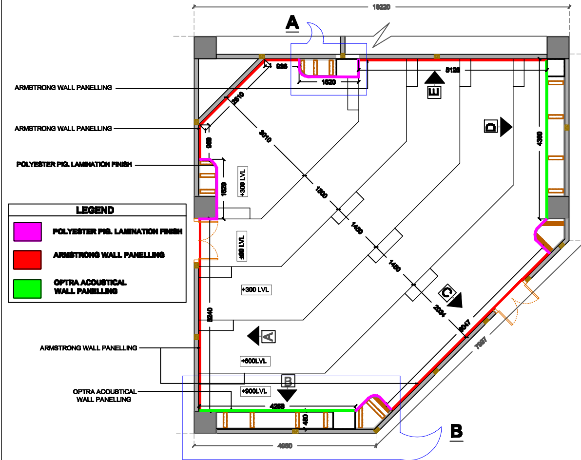
WALL PANELLING LAYOUT
