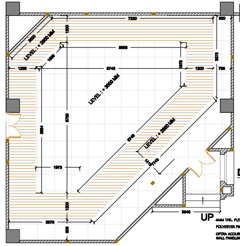
REFLECTED CELING PLAN
