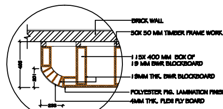
DETAIL OF X
