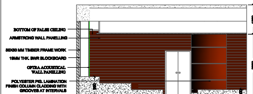
WALL ELEVATION A
