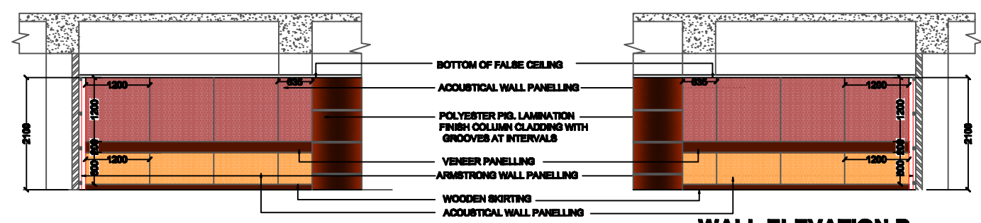
WALL ELEVATION D
